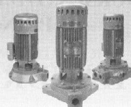
JET PUMPS
